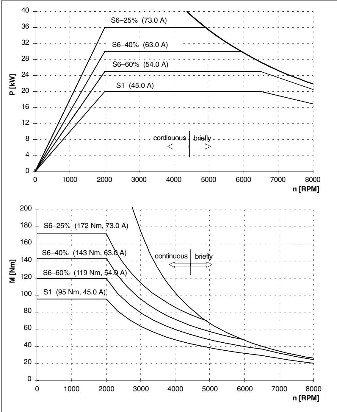
Fig. 2-23 1PH7133-□NG□□
