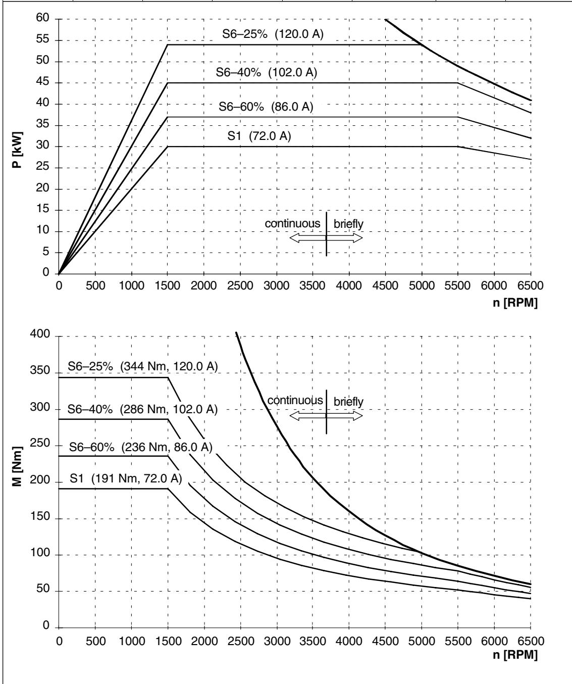
Fig. 2-37 1PH7163-□NF□□
