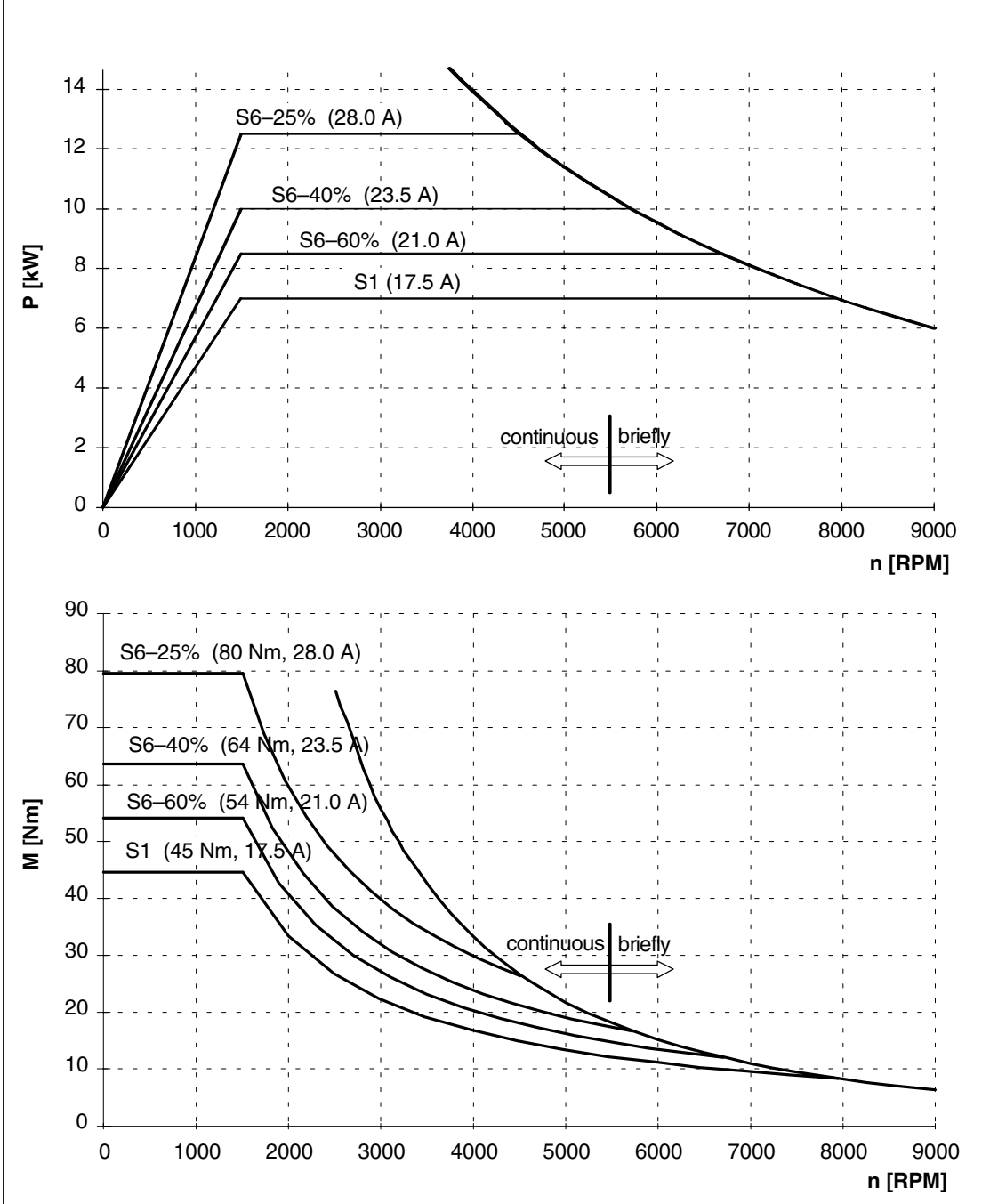
Fig. 2-9 1PH7105-□NF□□
