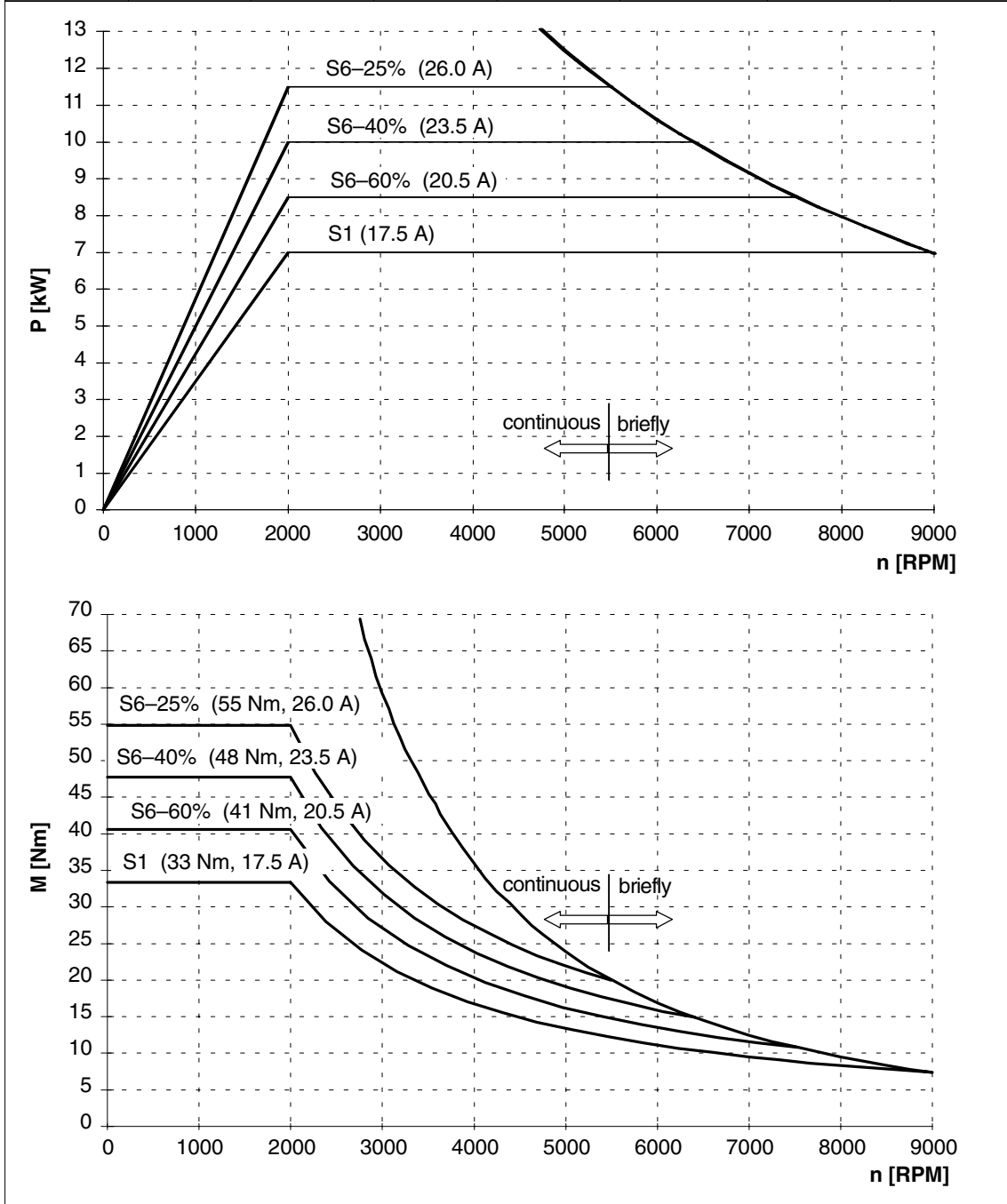
Fig. 2-7 1PH7103-□NG□□
