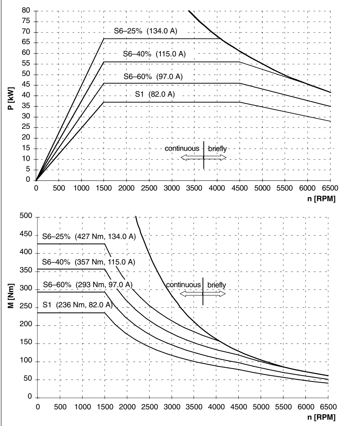
Fig. 2-45 1PH7167-□NF□□
