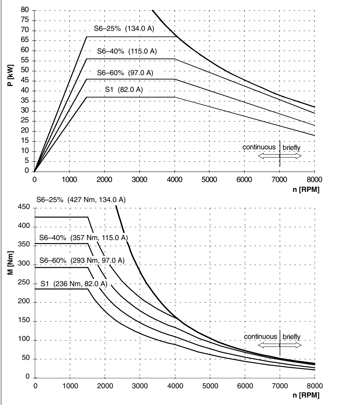
Fig. 2-46 1PH7167-□NF□□-0L
