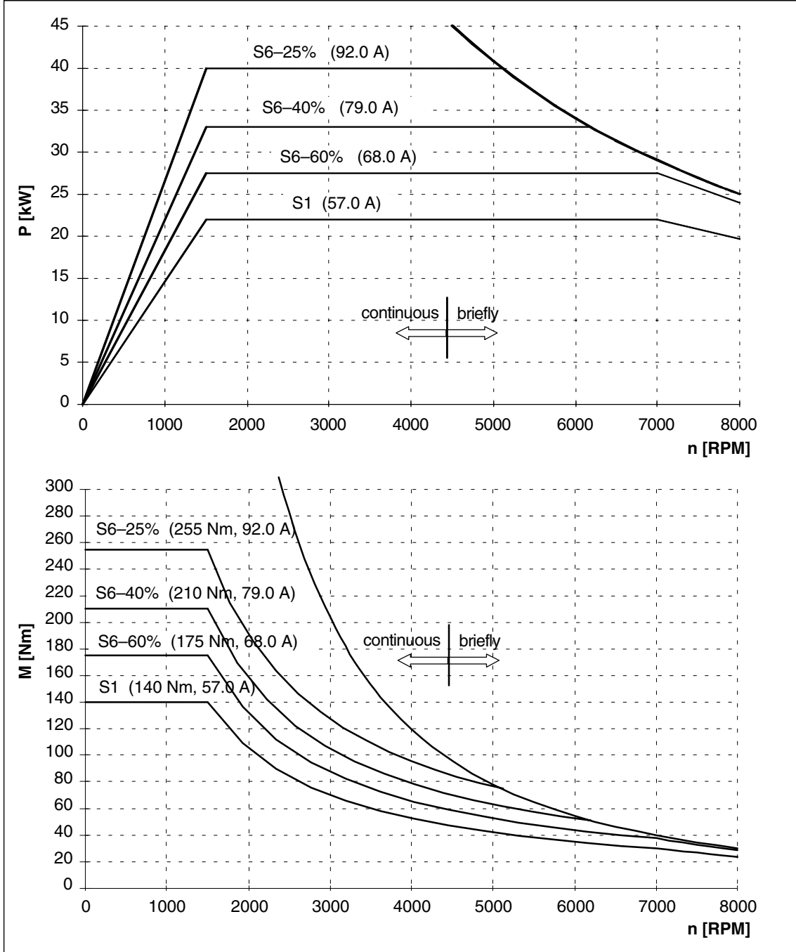
Fig. 2-29 1PH7137-□NF□□
