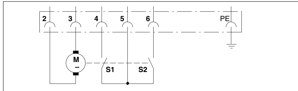
Fig. 3-5 Circuit diagram
