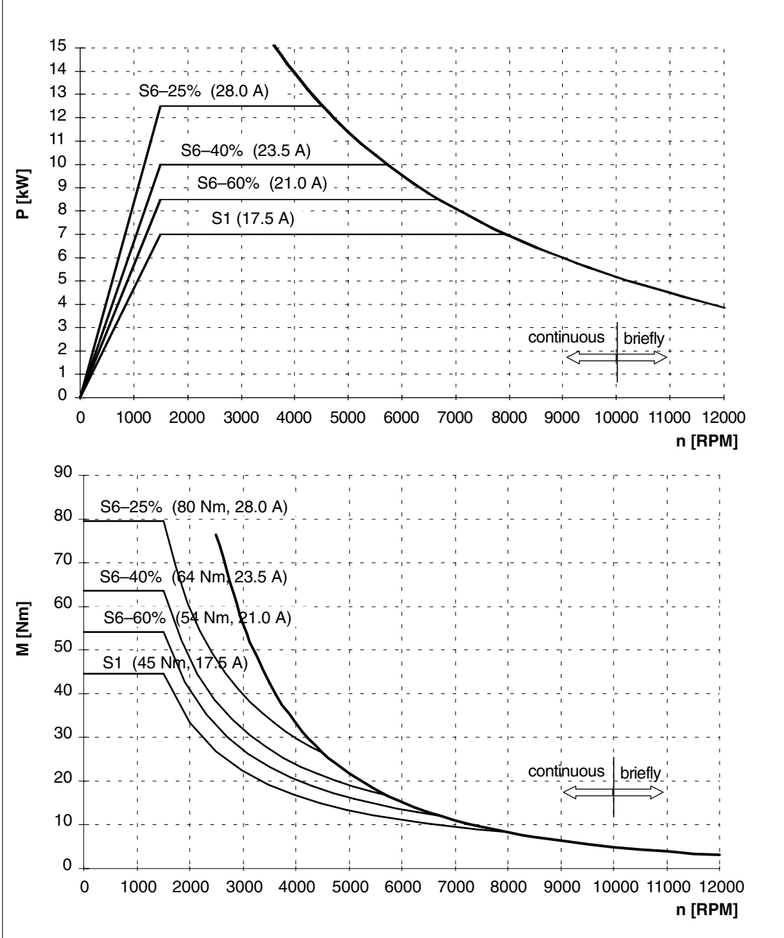
Fig. 2-10 1PH7105-□NF□□-0L
