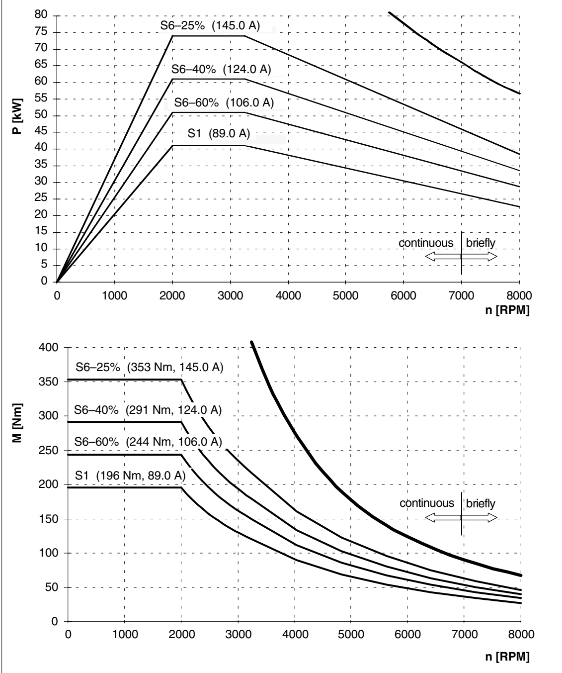
Fig. 2-48 1PH7167-□NG□□-0L
