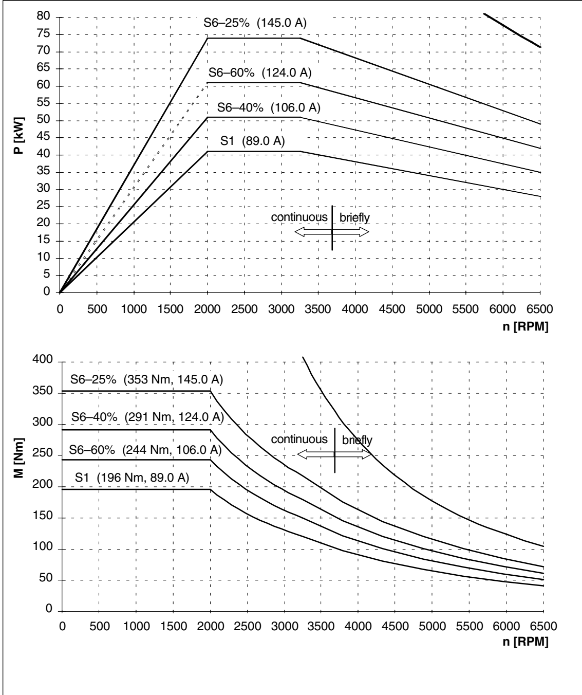
Fig. 2-47 1PH7167-□NG
